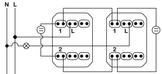
2-module - Two way switch with locator lamp
