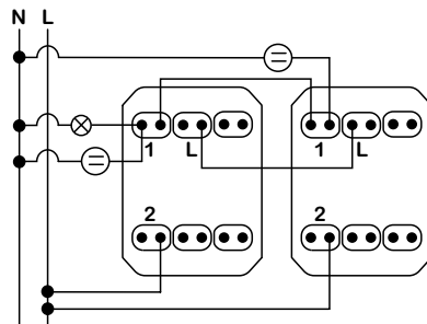
2-module - 2 two-way switches with indicator lamp
