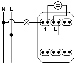
2-module - One-way switch with locator lamp
