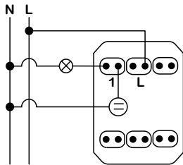
1-module - One-way switch with indicator lamp
