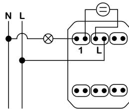
2-module - Push button with locator lamp
