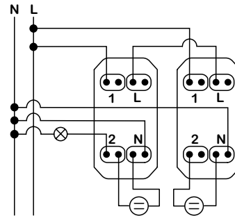
1-module - 2 two-way switches with indicator lamp and neutral connection
