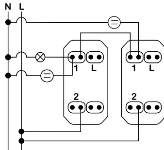
1-module - 2 two-way switches with indicator lamp
