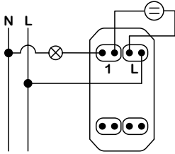
1-module - One-way switch and push button with locator lamp
