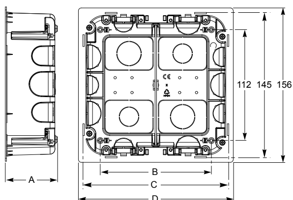
Vertical flush centralization boxes
