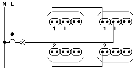
2-module - Two-way switch
