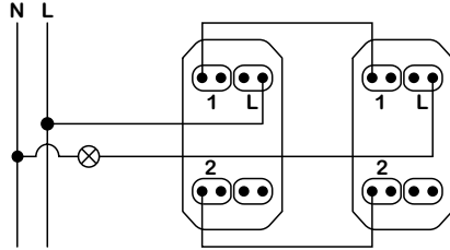
1-module - 2 two-way switches
