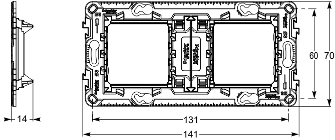
Plastic (2-gang or 4-module)
