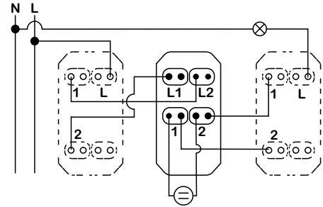
1-module - 2 two-way switches + 1 intermediate with locator lamp
