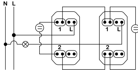
1-module - 2 two-way switches with locator lamp
