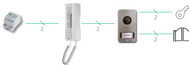
1122/31 wiring diagrams (options) automatic gate
